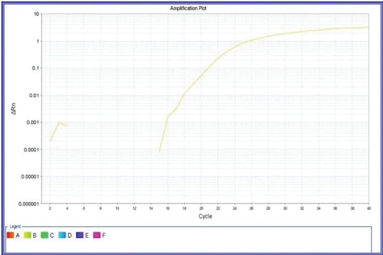
Positive Mycoplasma pneumoniae control curve.
