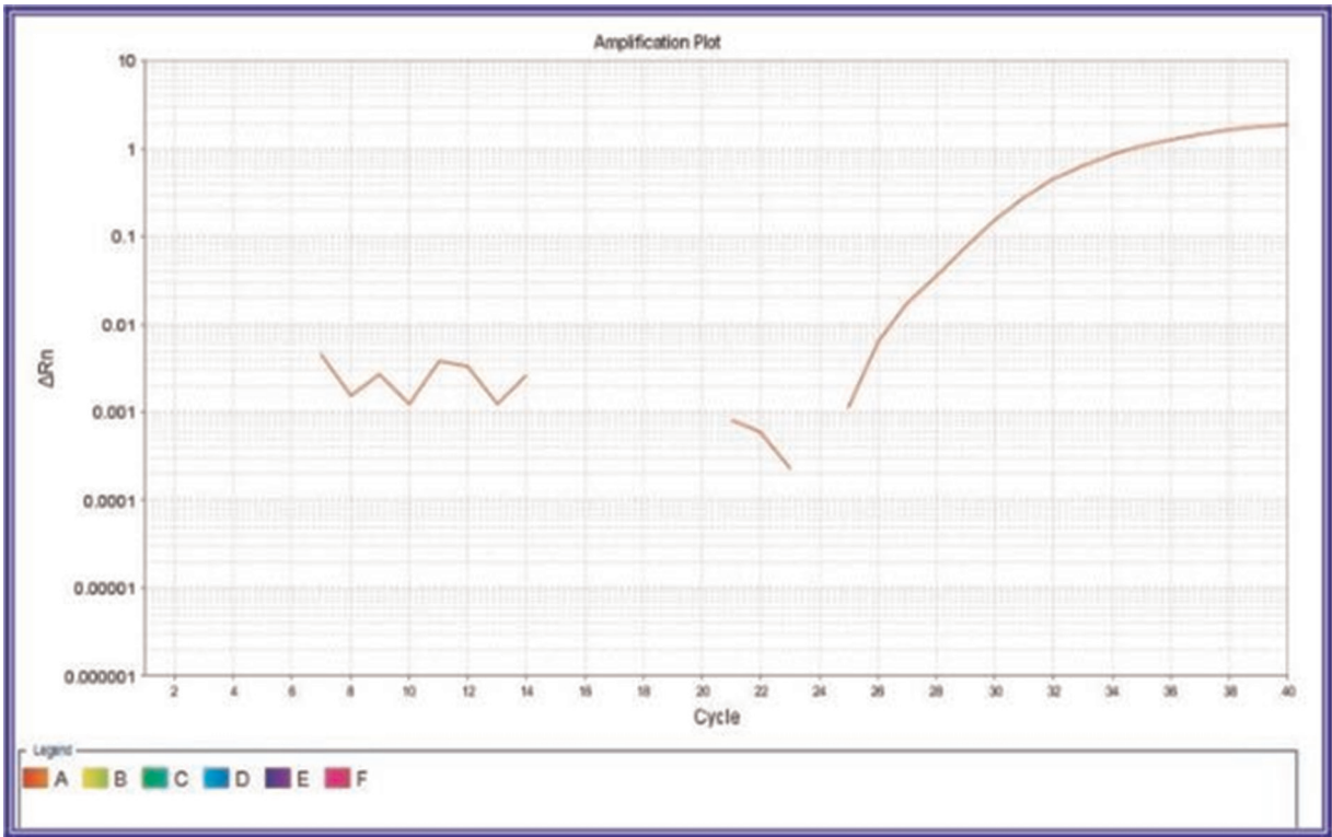
Positive result curve shows amplification.
